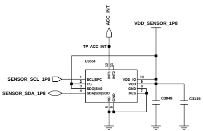
Accel. Sensor
