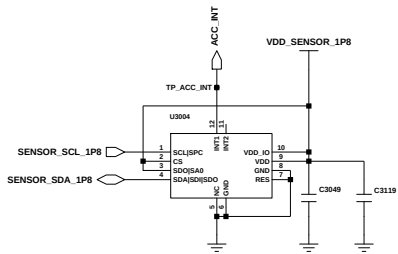
Accel. Sensor
