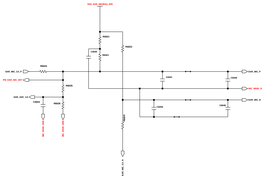
Ear MIC
