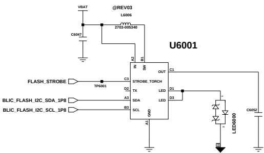
FLASH LED driver IC(new item) COPY FROM A135F
