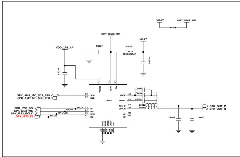
SPK AMP NEW
